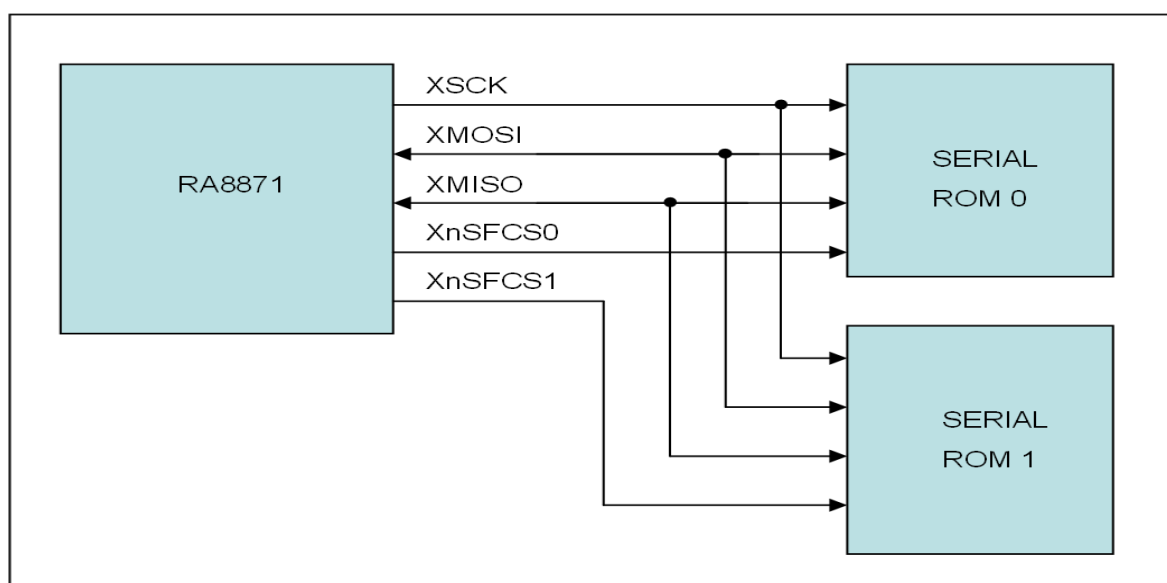
Figure 3.3: RA8871M Serial Flash/ROM System
