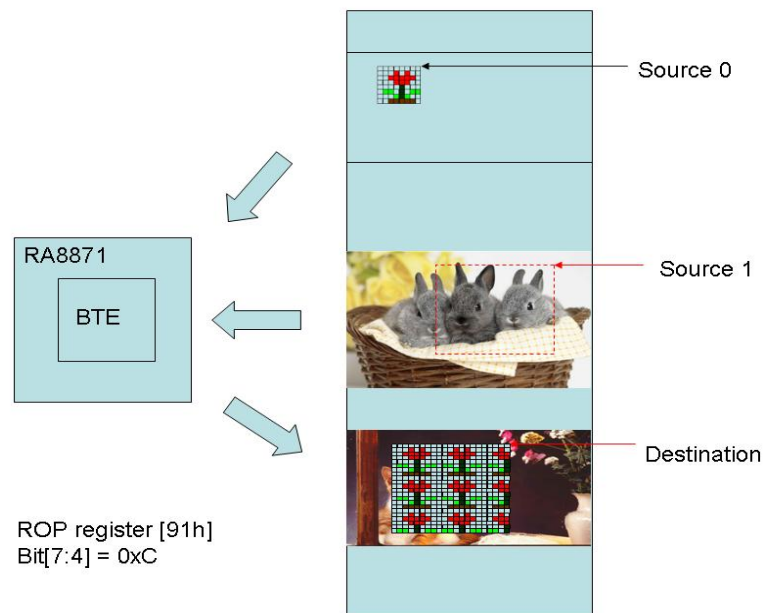
Figure 4-72 : Hardware Data Flow
