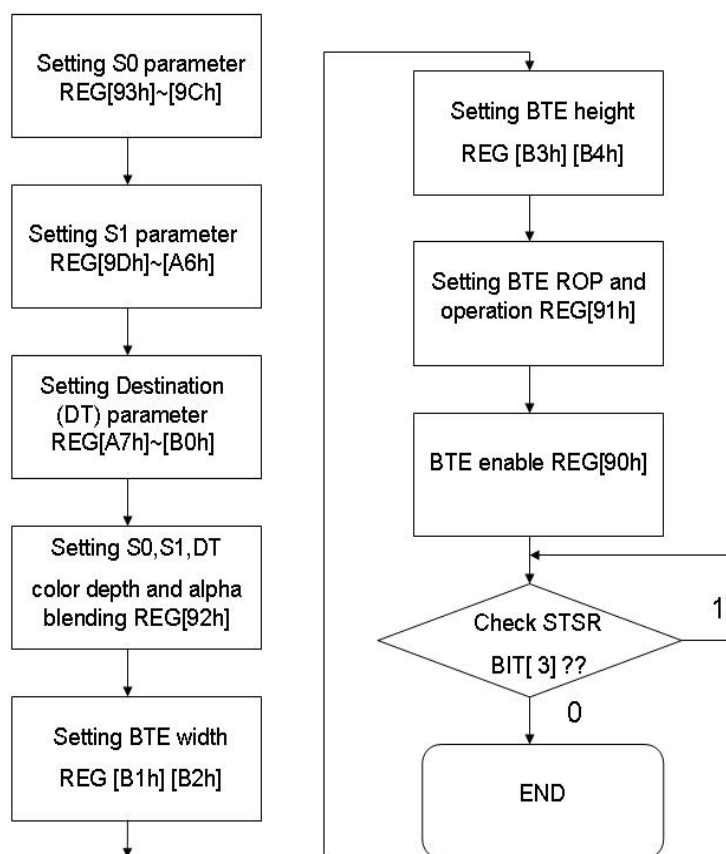
Figure 4-6 : Flow Chart
