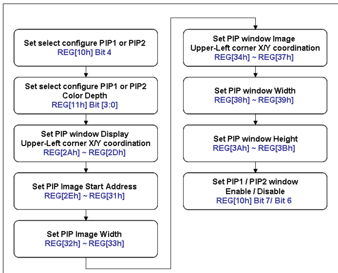
Figure 5-1 Flow Char
